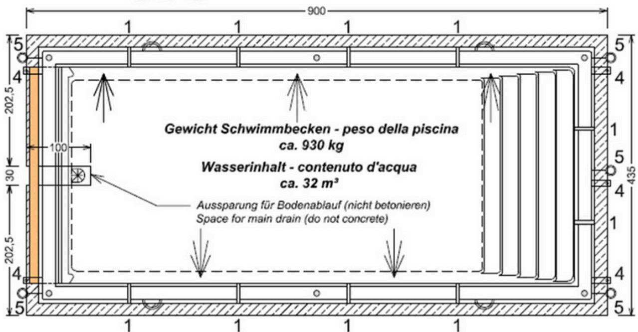
Grundriss - Ground plan
